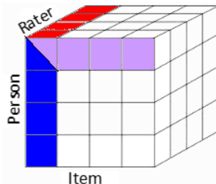
rows = person columns = items 3rd dimension (slices) = raters
