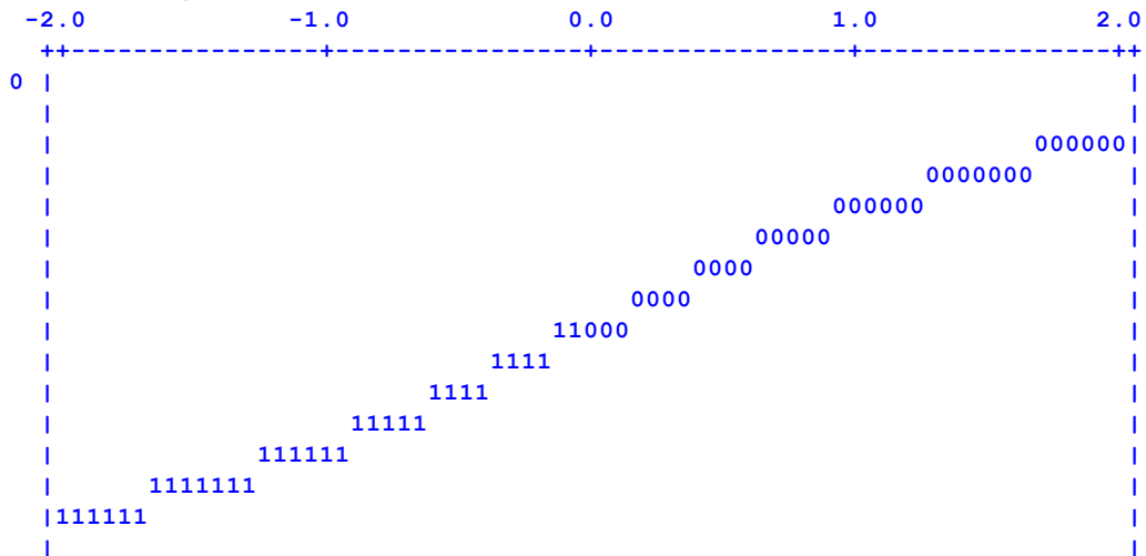
Expected Score Ogive (Model ICC)
